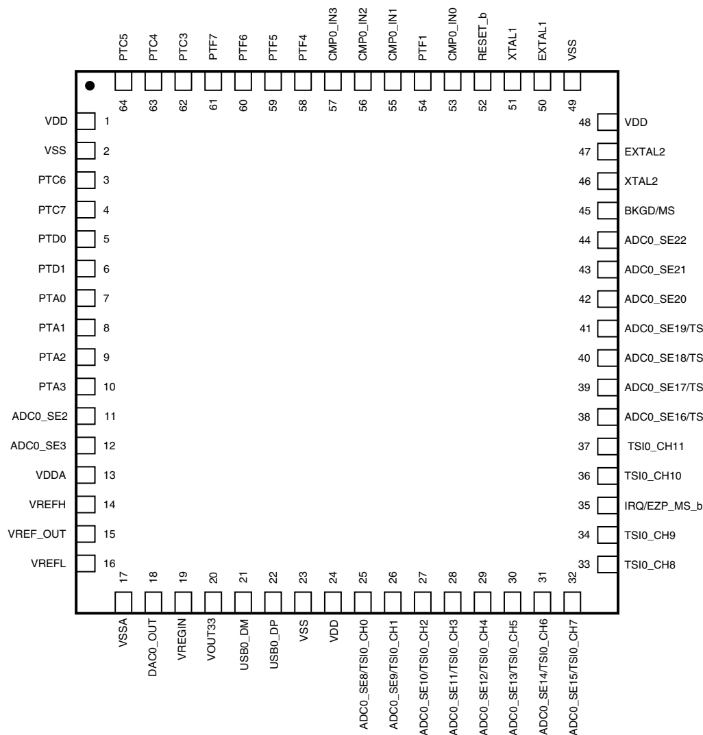
Figure 20. 64-pin LQFP
