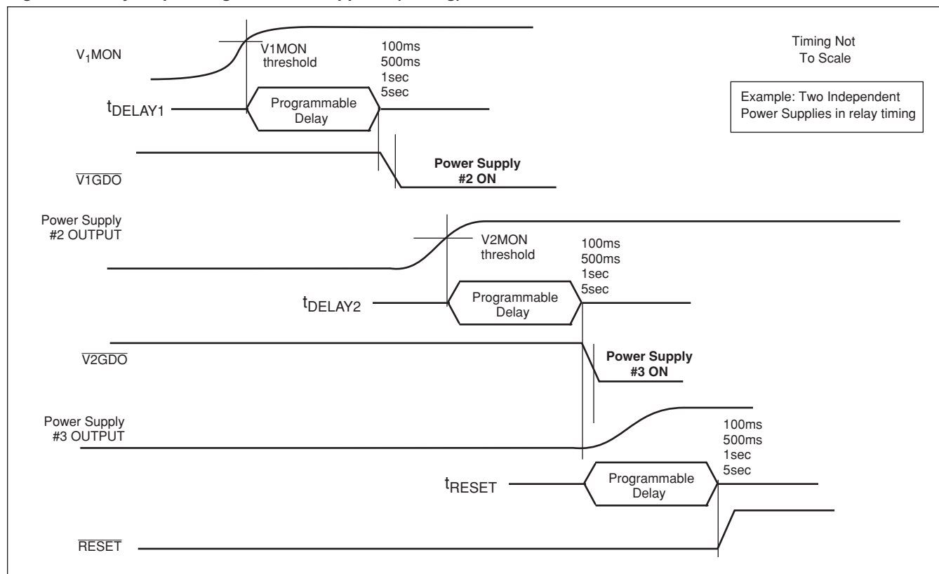
Figure 10. Relay Sequencing of DC-DC Supplies. (Timing)
