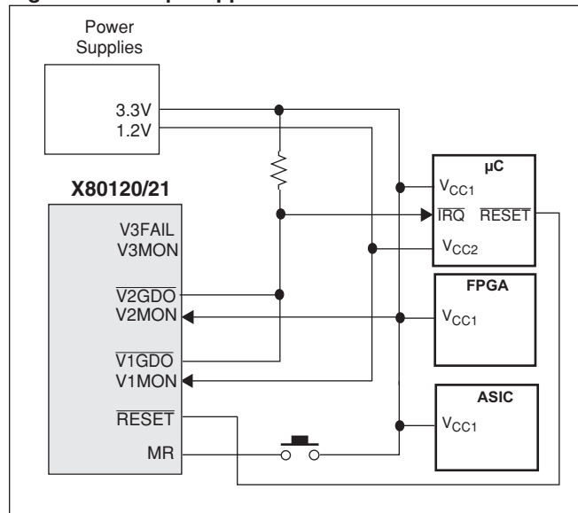
Figure 7. Example Application of Parallel Power Control.
