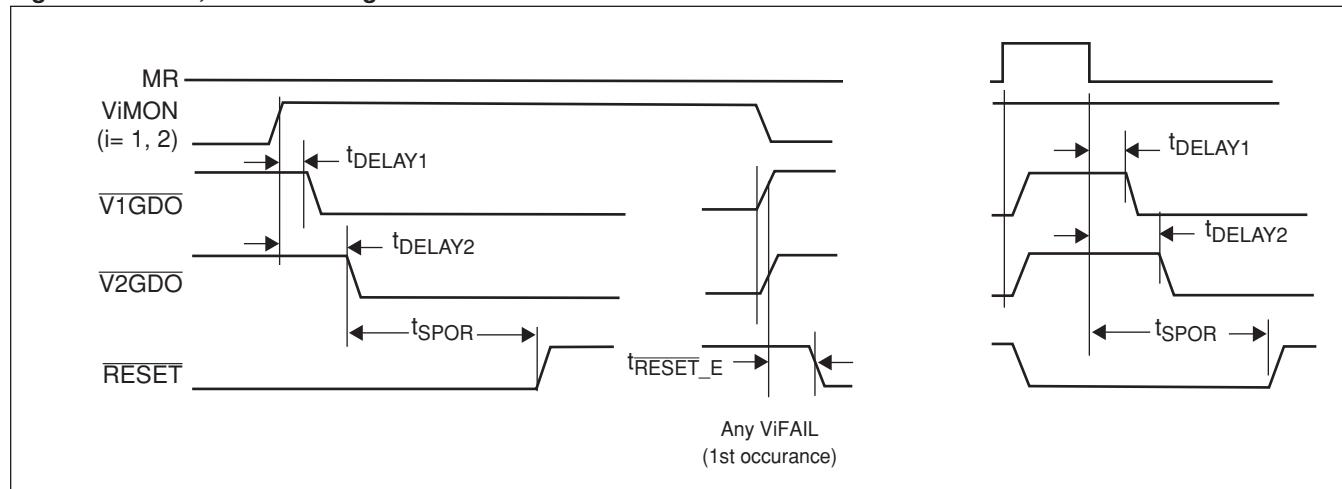
Figure 3. ViFAIL, RESET Timings
