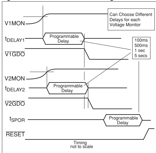
Figure 8. Parallel Power Control - Timing
