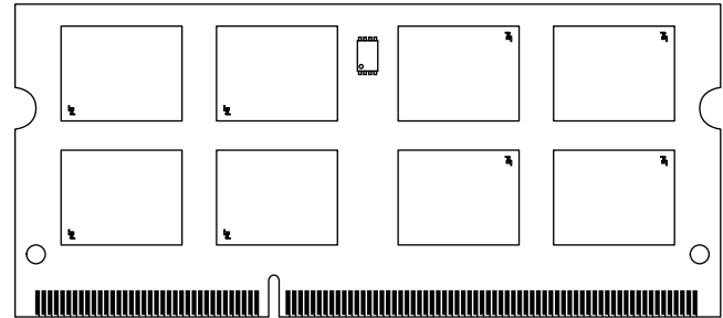
Figure 1: 204-Pin SODIMM (MO-268 R/C F)
