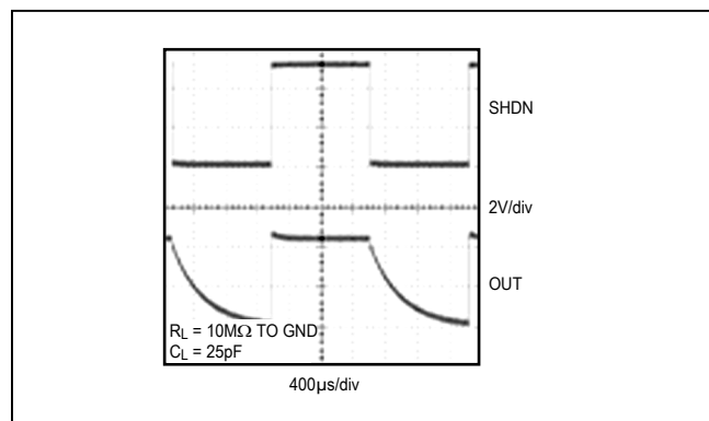
Figure 4. Shutdown Waveform
