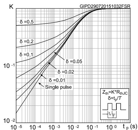
Figure 17. Thermal impedance
