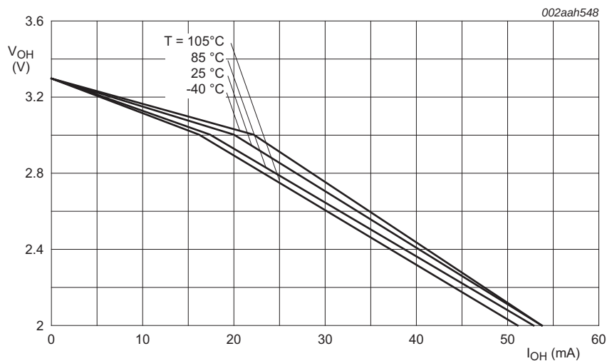
Fig 36. High-drive output: Typical HIGH-level output voltage V_{OH} versus HIGH-level output current I_{OH} .
