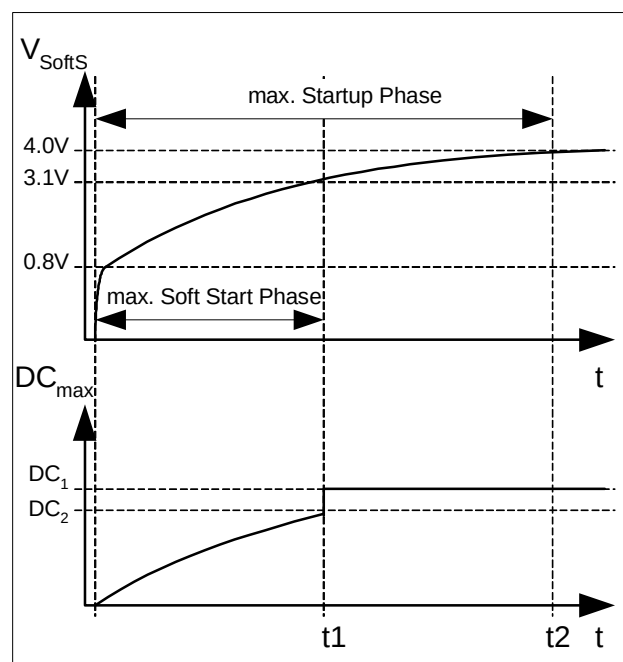
Figure 5 Startup Phase
