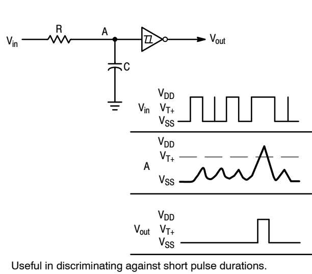
Figure 6. Integrator
