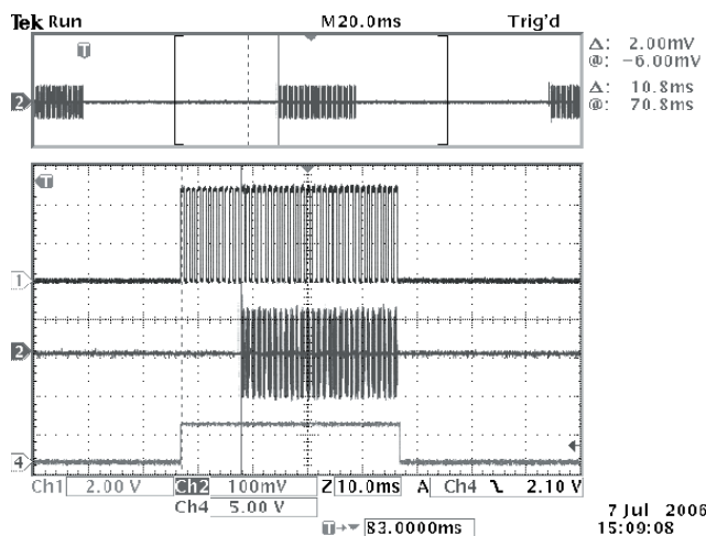
Figure 4. RF Out after shut down cycle example (11ms) Ch 1 - ASK pin, 1ms period Ch 2 RF Field, ch 4 - Standby Pin
