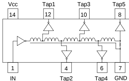
AIDM 14-Pin Schematic
