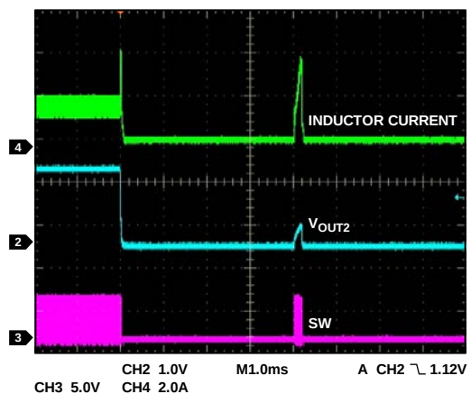
Figure 54. Current Limit Entry, Channel 2 V_{OUT} = 1.8 \text{ V} , 2 A Configuration, f_{SW} = 600 \text{ kHz}
