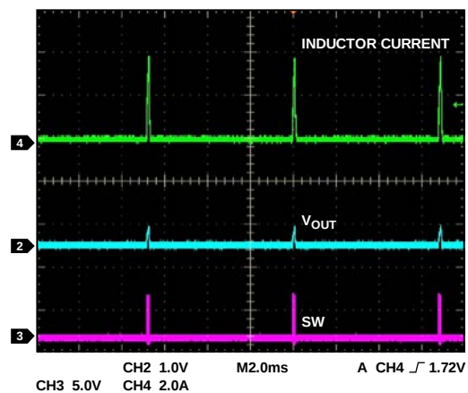
Figure 56. Hiccup Mode, f_{SW} = 600 \text{ kHz} , 6.8 ms Hiccup Cycle
