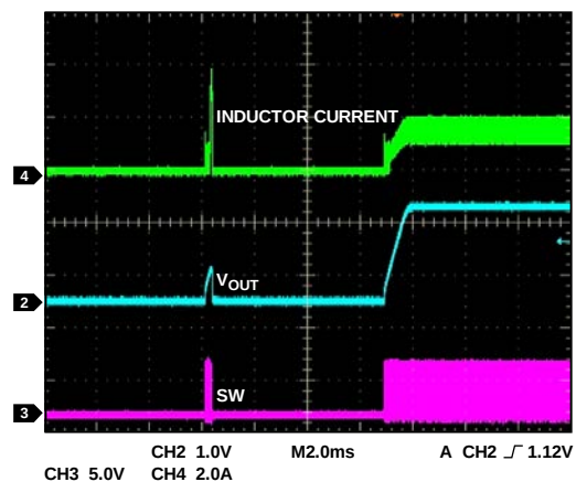
Figure 57. Exit Hiccup Mode, Channel 2 V_{OUT} = 1.8 \text{ V} , f_{SW} = 600 \text{ kHz}
