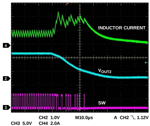
Figure 55. Current Limit Entry (Zoomed In), Channel 2 V_{OUT} = 1.8 \text{ V} , 2 A Configuration, f_{SW} = 600 \text{ kHz}
