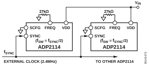
Figure 73. Synchronization with External Clock ( f_{SW} = 1.2 \text{ MHz} in This Case)
