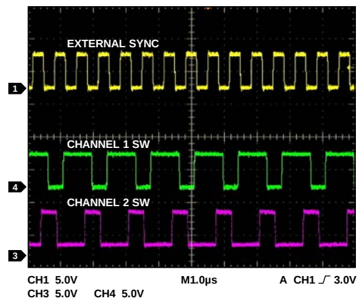
Figure 58. External Synchronization, f_{SYNC} = 1.5 \text{ MHz} , f_{SW} = 750 \text{ kHz}
