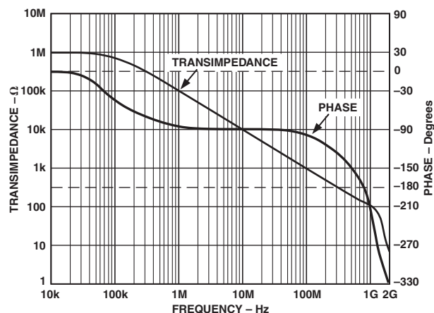
TPC 10. Transimpedance and Phase vs. Frequency
