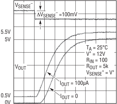
Step Response Rising Edge
