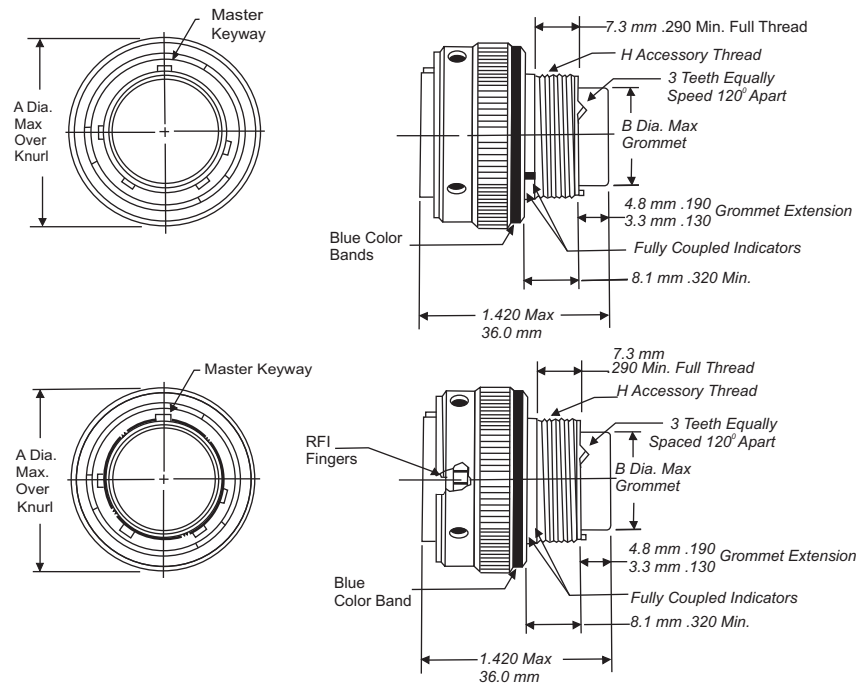
Plug Shell, Bayonet Coupling Military No. MS3476
