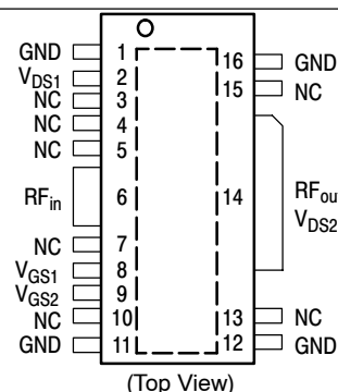
Figure 2. Pin Connections
