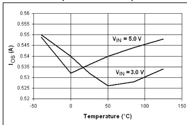
Figure 48. I_{OS} vs. temperature (STMP2161/2171)
