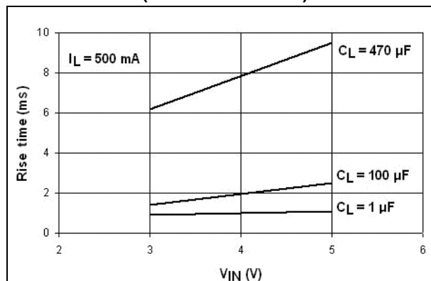
Figure 50. Output rise time vs. V_{IN} (STMP2161/2171)
