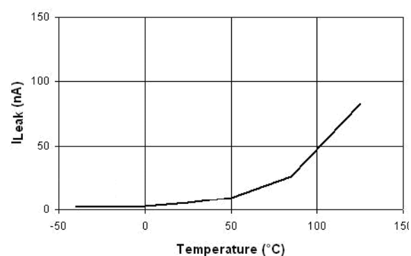
Figure 49. Switch leakage vs. temperature (STMP2161/2171)
