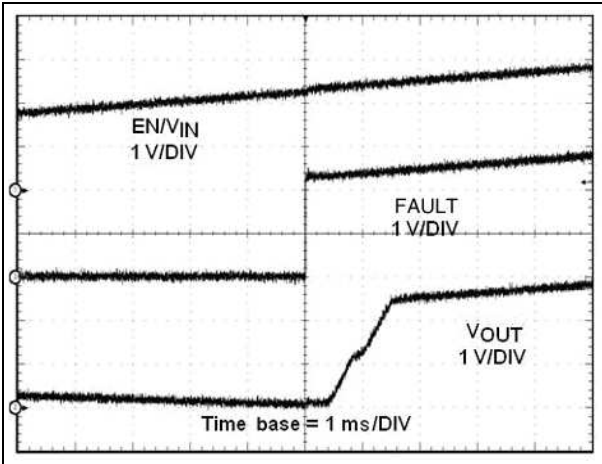
Figure 36. UVLO rising (STMP2161/2171)
