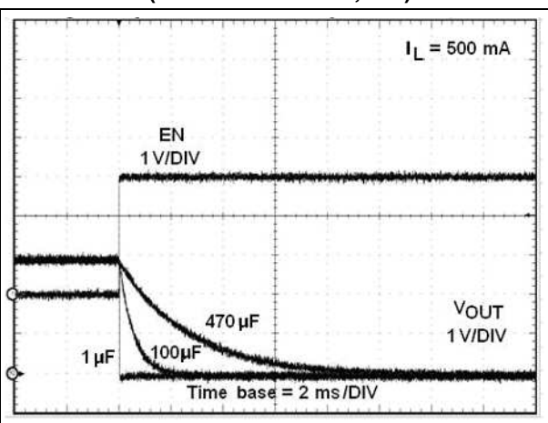
Figure 8. Voltage output turn-off delay time (STMP2141/2151, 3 V)
