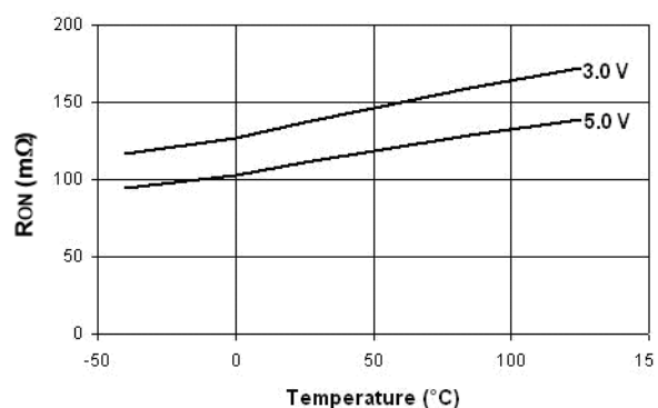
Figure 47. R_{ON} vs. temperature (STMP2161/2171)
