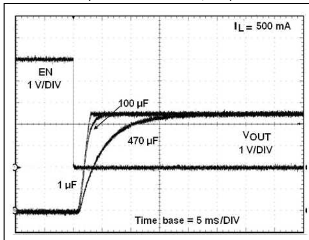
Figure 28. Voltage output turn-on delay time (STMP2161/2171, 5 V)
