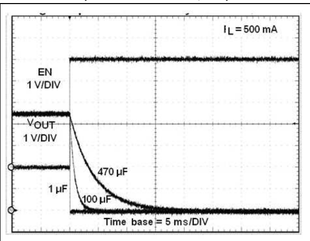
Figure 29. Voltage output turn-off delay time (STMP2161/2171, 5 V)
