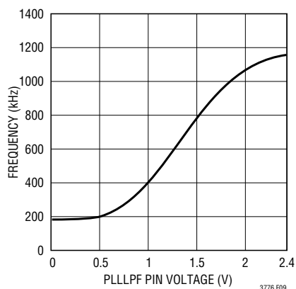
Figure 9. Relationship Between Oscillator Frequency and Voltage at the PLLPF Pin When Synchronizing to an External Clock
