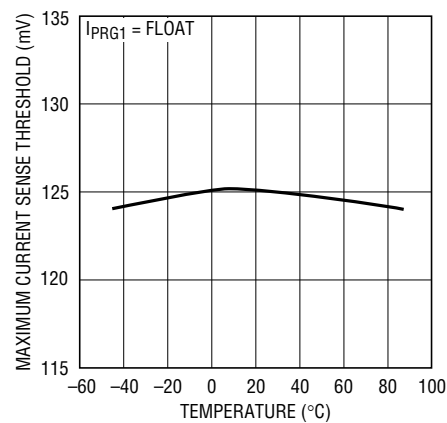
Maximum Current Sense Threshold (CH1) vs Temperature
