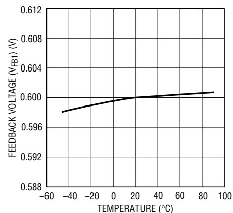
Regulated Feedback Voltage (CH1) vs Temperature
