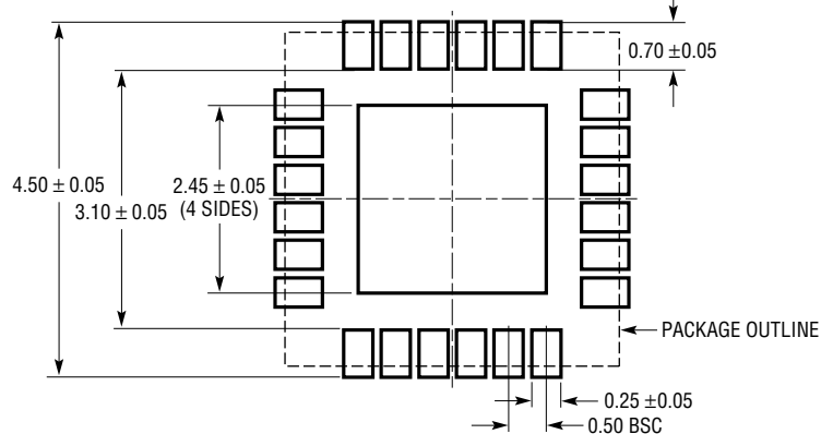
RECOMMENDED SOLDER PAD PITCH AND DIMENSIONS
