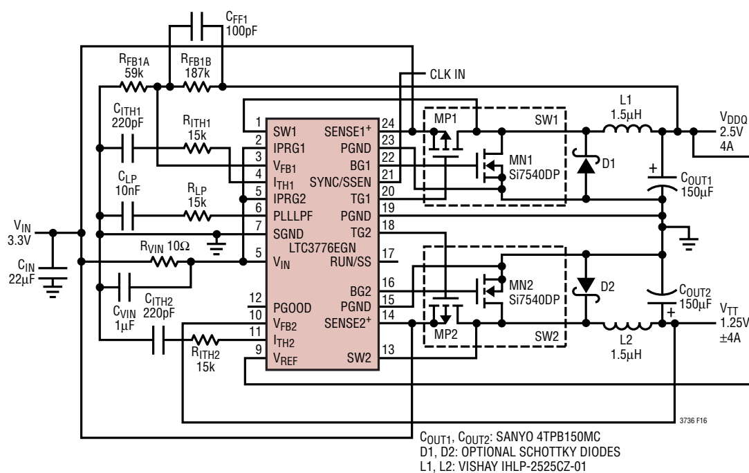
Figure 16. 2-Phase, Synchronizable, DDR Memory Supplies
