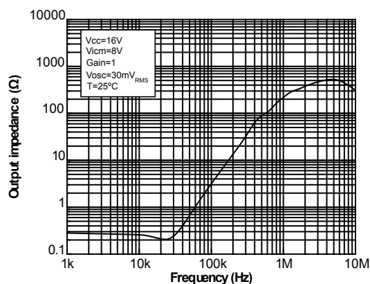
Figure 27. Output impedance vs. frequency in closed loop configuration
