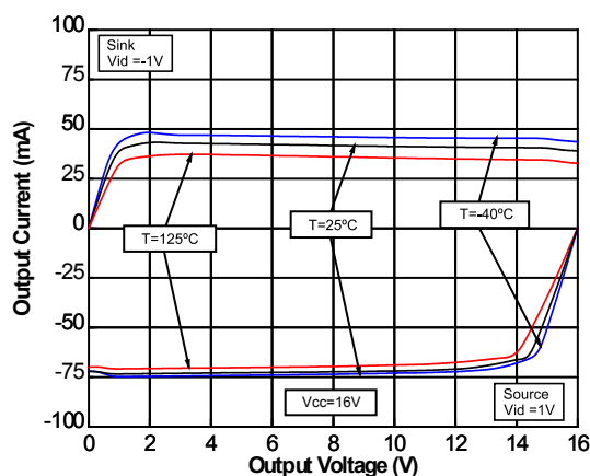
Figure 13. Output current vs. output voltage at V_{CC} = 16\text{ V} (TSX712)
