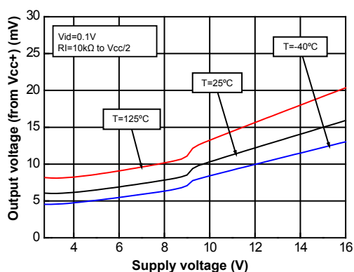
Figure 15. Output high voltage (drop from V_{CC+} ) vs. supply voltage
