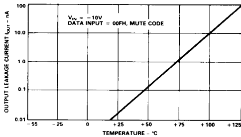
Figure 12. Typical Output Leakage Current vs. Temperature
