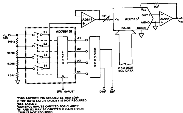
Figure 8. 0 to 80dB Attenuator with 0.1dB Resolution
