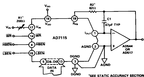
Figure 4. Typical Circuit Configuration
