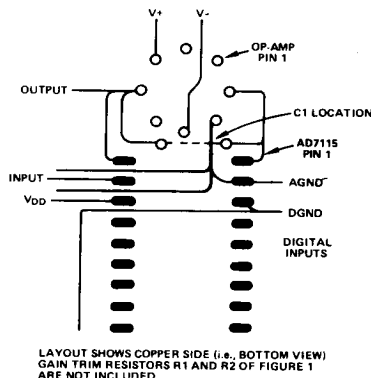
Figure 5. Suggested Layout for AD7115 and Op-Amp (Not to Scale)
