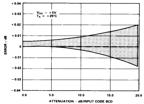
Figure 13. Typical Attenuation Error vs. Attenuation/Input Code
