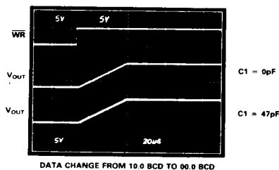
Figure 6. Response of AD7115 with AD517
