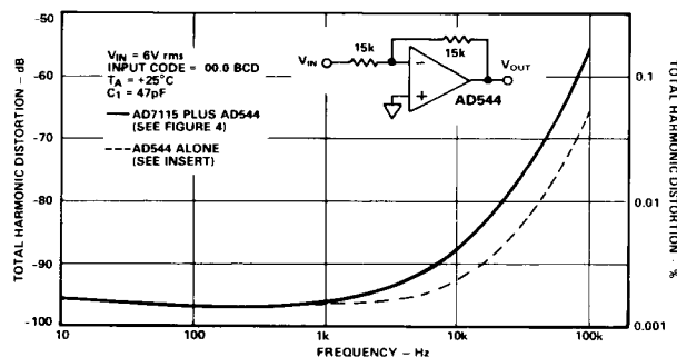
Figure 14. Typical Distortion vs. Frequency Using AD544 Amplifier
