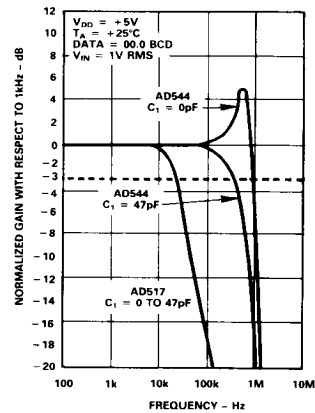
Figure 11. Frequency Response with AD544 and AD517 Amplifiers
