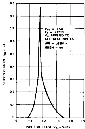
Figure 10. Typical Supply Current vs. Logic Input Level
