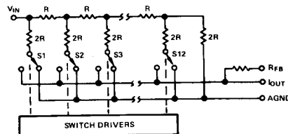
Figure 2. Simplified D/A Circuit of AD7115
