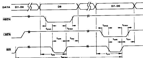
Figure 1. Data Loading Waveforms with 8-Bit Data Bus
