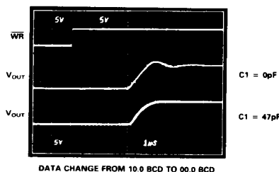
Figure 7. Response of AD7115 with AD544
