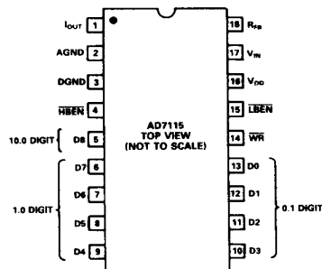
PIN CONFIGURATION
