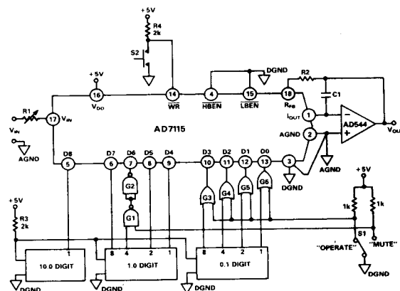
Figure 9. Thumbwheel Switch Attenuator
