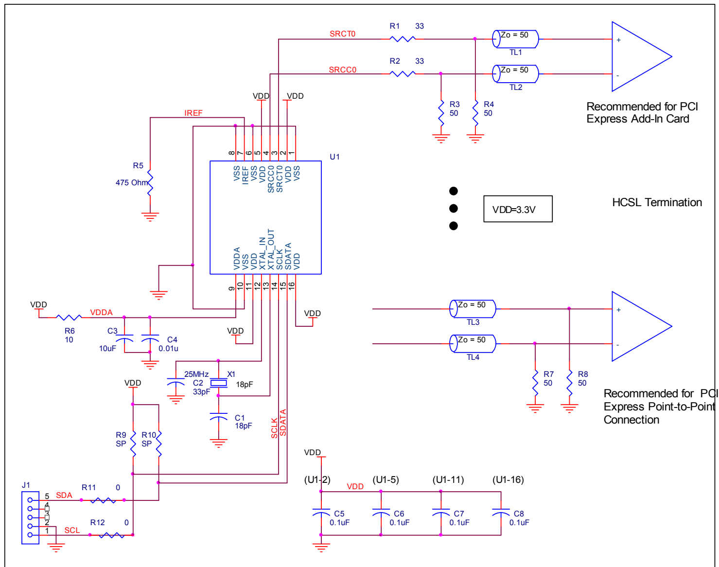
Figure 5. ICS841S101I Application Schematic.
