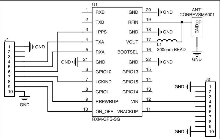
Figure 3: MDEV-GPS-SG-DB Schematic
