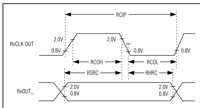
Figure 5b. MAX9236/MAX9238 Output Setup/Hold and High/Low Times
