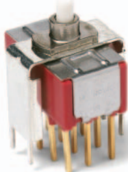
8421SD3_GE 4PDT
