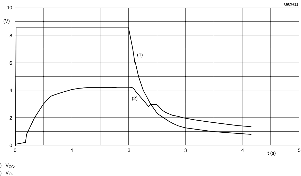
Fig.15 Turn-on/off behaviour.
