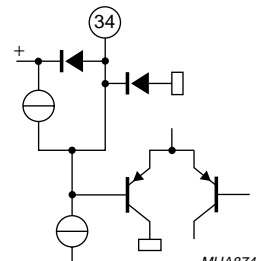
Fig.44 Pin 34: capacitor for filter adjust.
