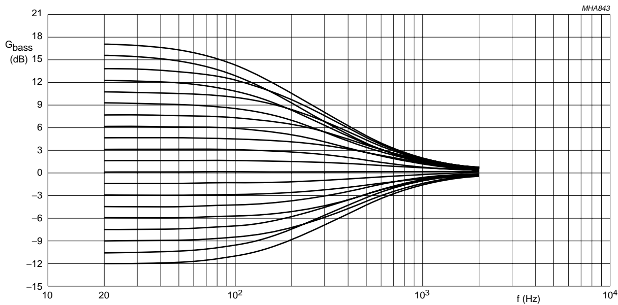
Fig.7 Bass control.
