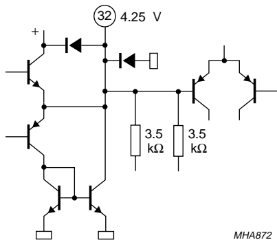
Fig.42 Pin 32: capacitor for pilot detector.
