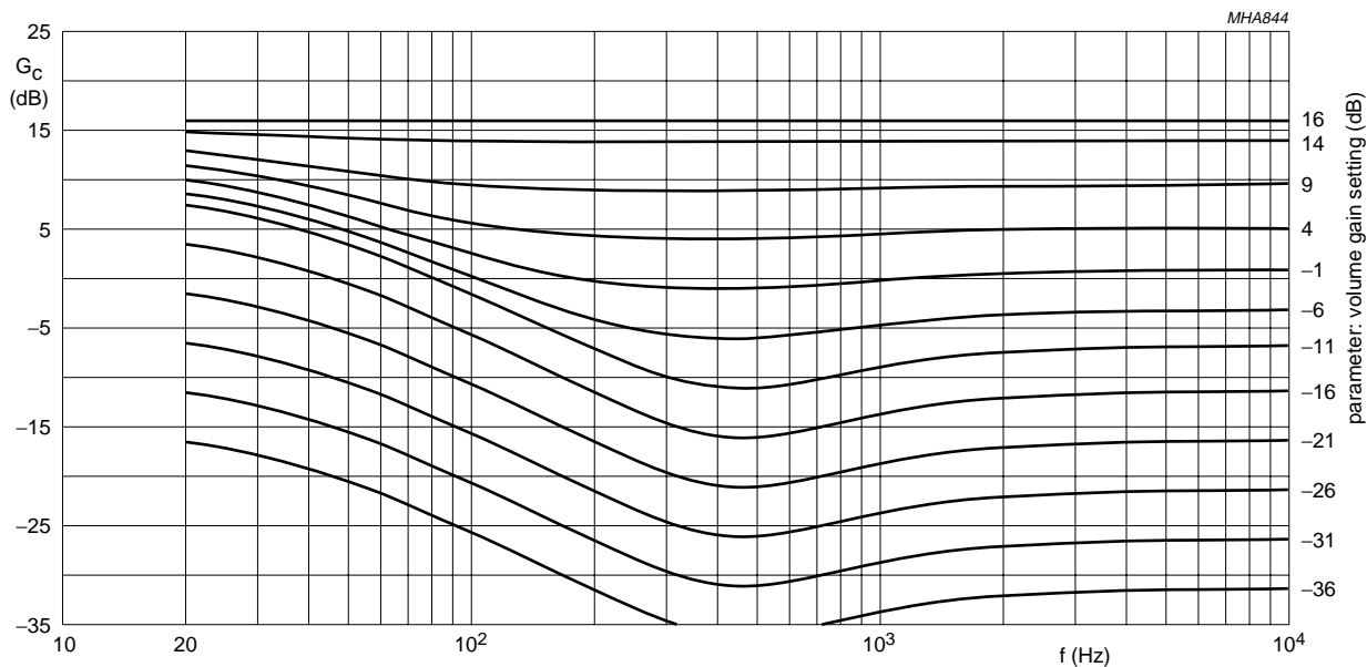
Fig.6 Volume control with loudness (including low roll-off frequency).
