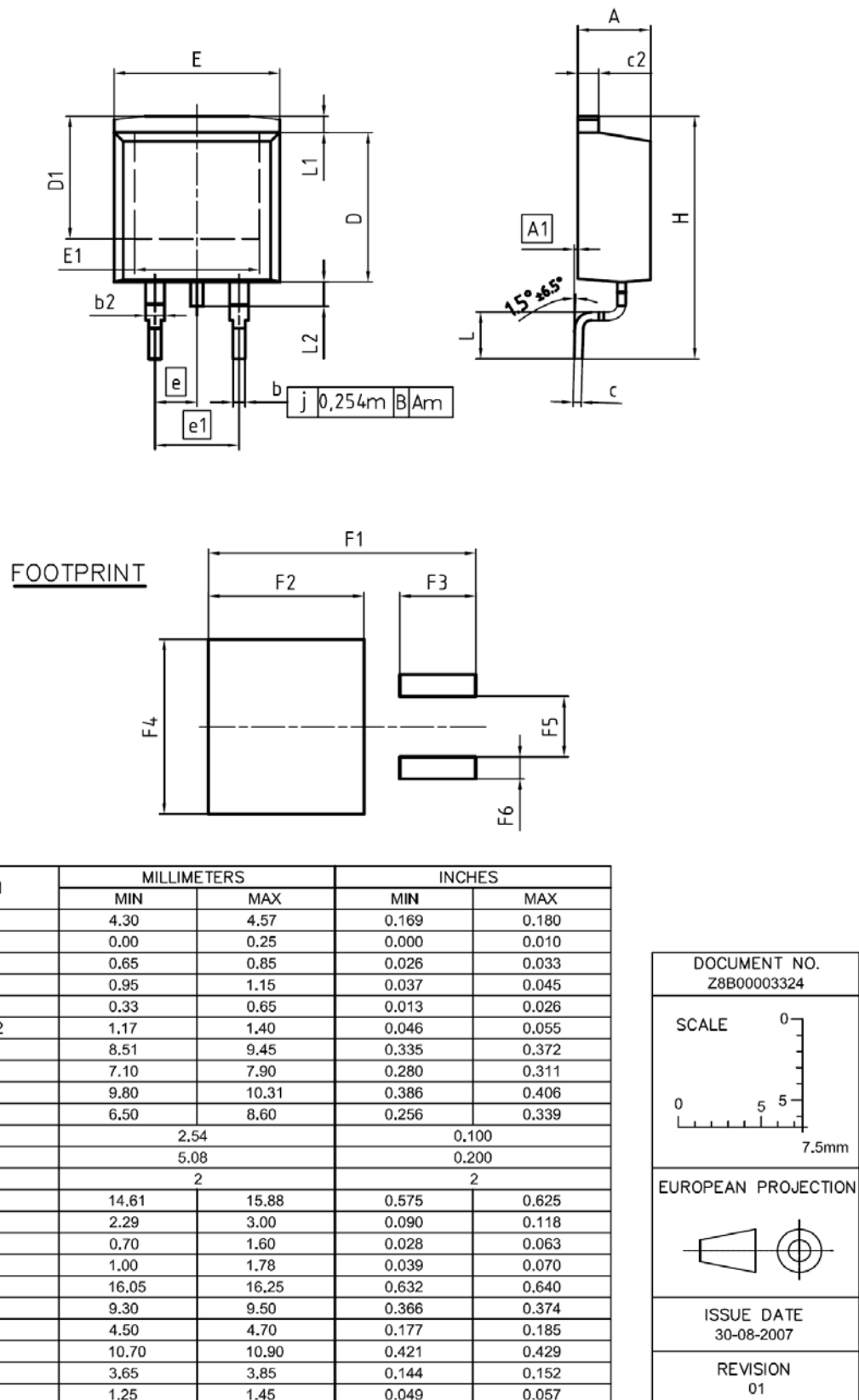
Figure 5 Outlines TO-263, dimensions in mm/inches
