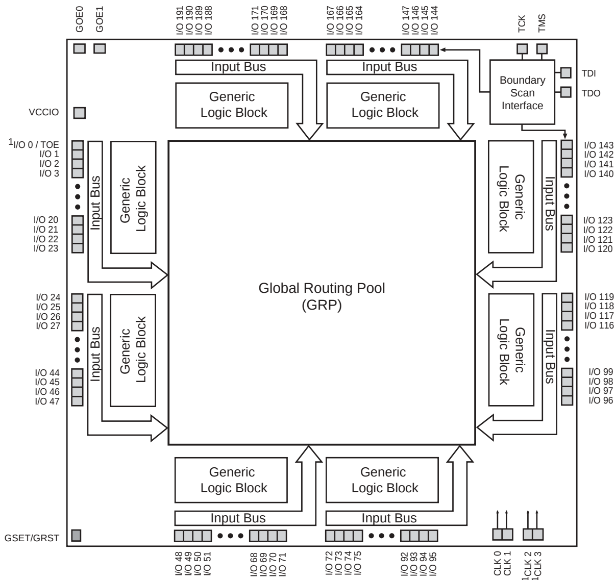
Figure 1. ispLSI 5256VA Functional Block Diagram (272 BGA Option)
