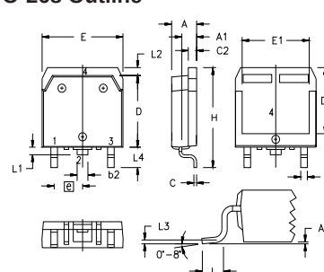
TO-268 Outline
