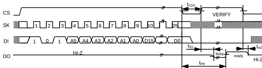
Figure 7 WRITE Timing (S-93C46A)
