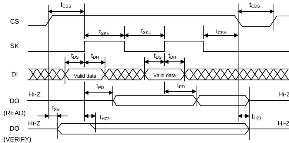
Figure 3 Read Timing
