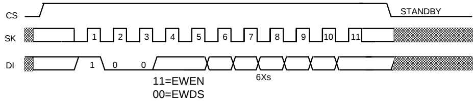
Figure 20 EWEN/EWDS Timing (S-93C56A)
