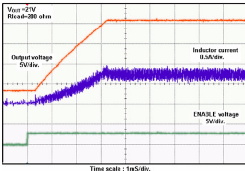
Figure 4: Start-Up Waveform
