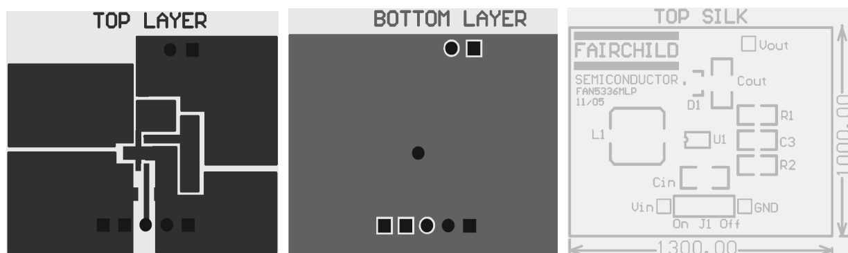
Figure 3: PCB Layout
