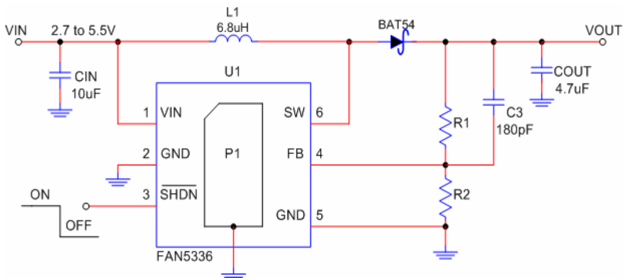
Figure 2: Schematic Diagram
