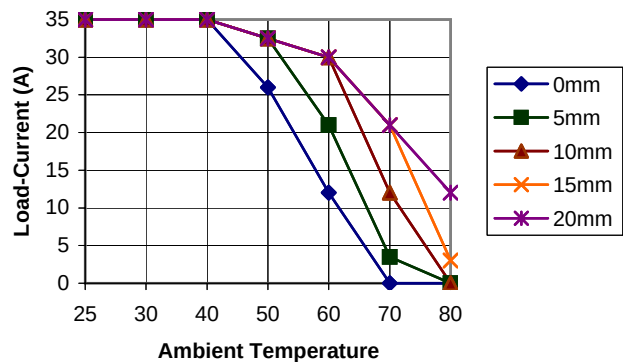
GNR45mm 35A Allowable Load-Current (Horizontal Spacing)
