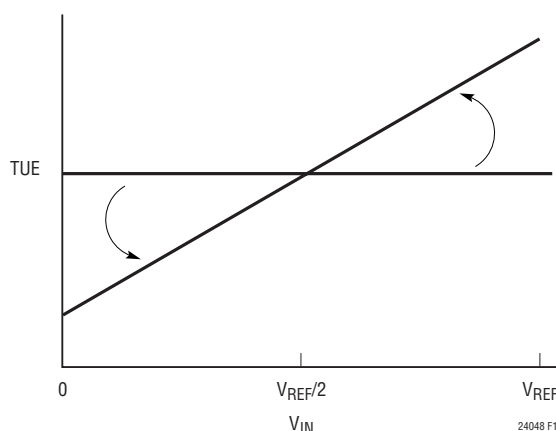
Figure 13. Offset/Full-Scale Shift
