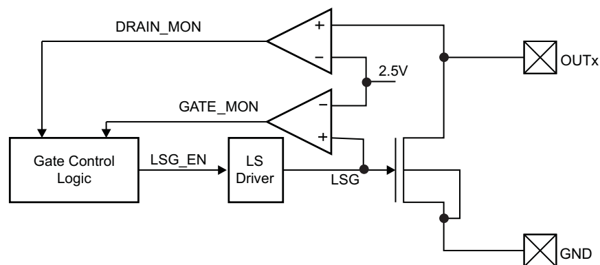
Figure 42. Low-Side Drive Schematic
