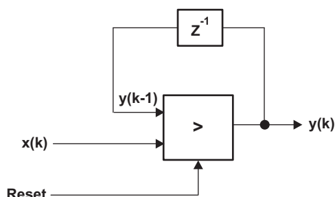
Figure 18. Peak Extractor
