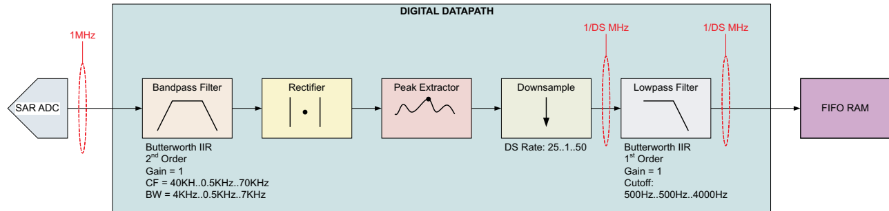
Figure 17. Digital Data Path
