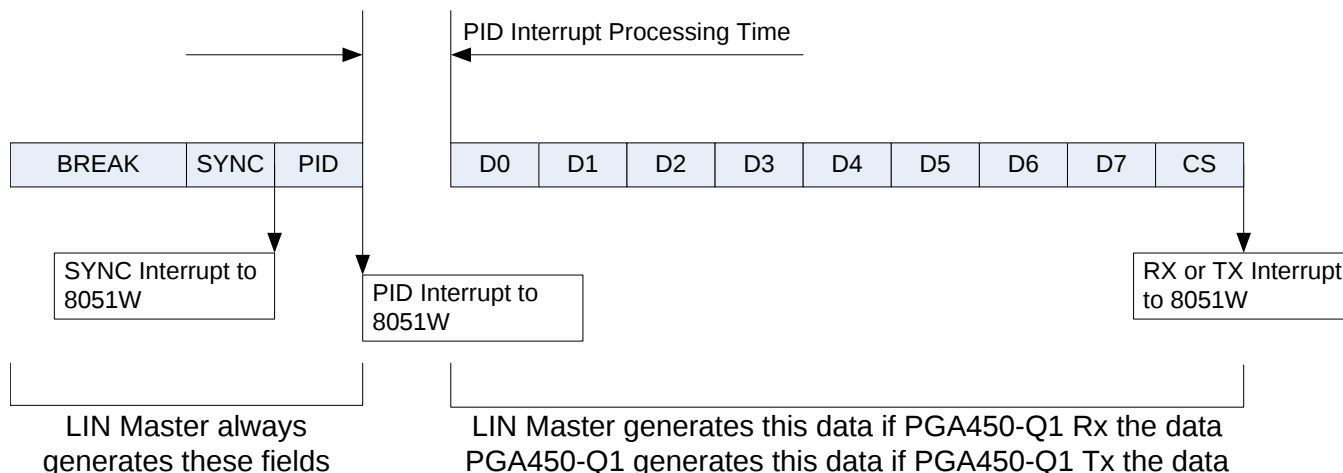
Figure 34. LIN Interrupts
