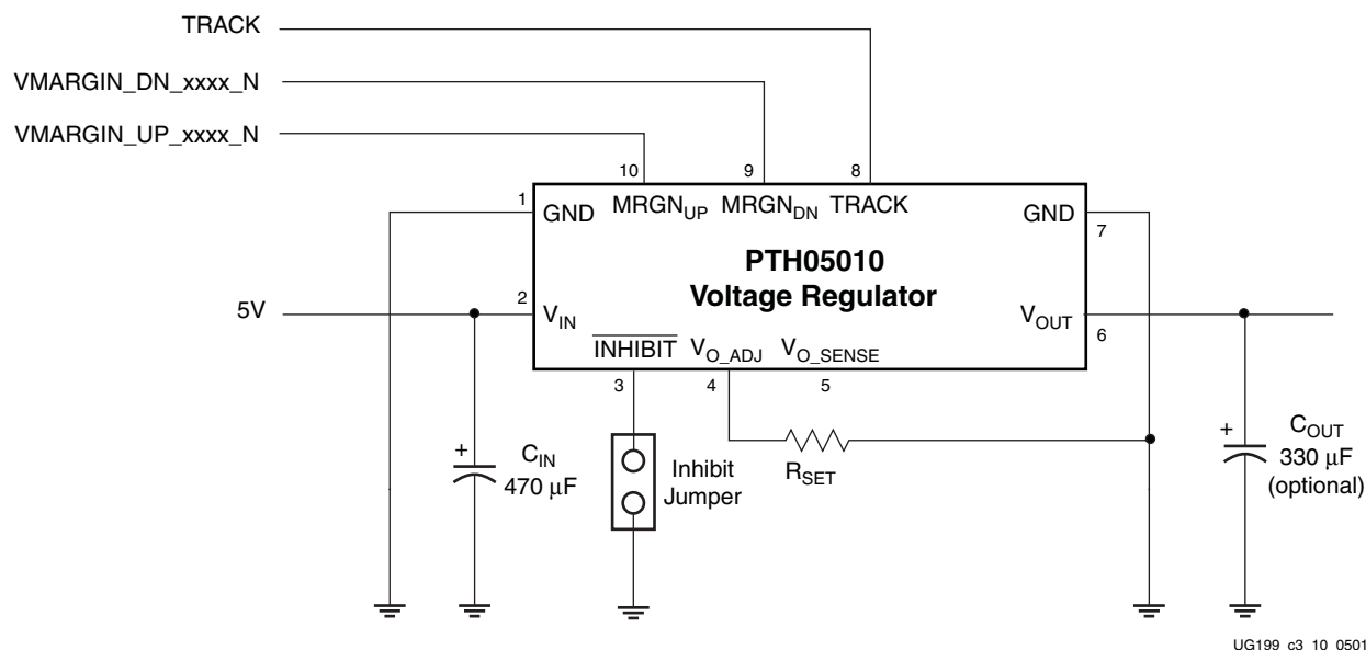
Figure 3-10: PTH05010 Voltage Regulator
