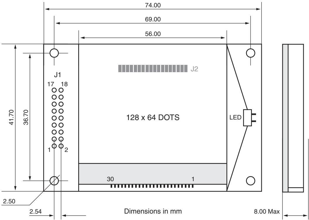
Figure C-4: 64128EFCBC-XLP Dimensions
