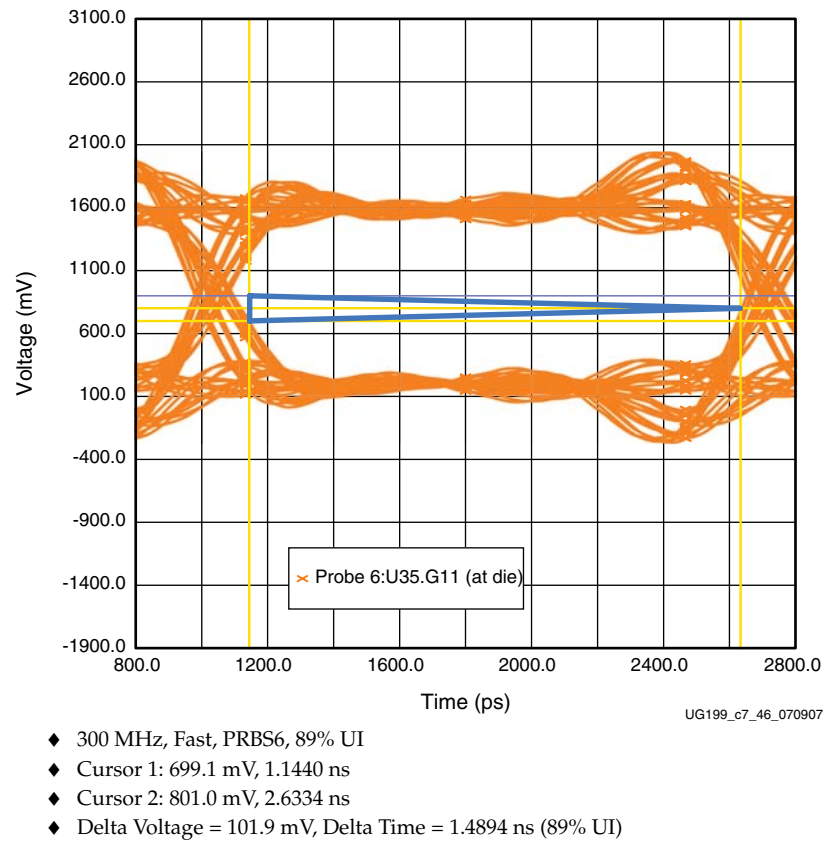
Figure 7-46: QDRII Write Extrapolation - Eye Scope Shot at Receiver IOB (Fast Corner)
