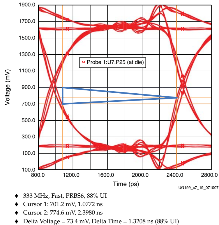
Figure 7-19: DDR2 Component Read Extrapolation - Eye Scope Shot at Receiver IOB (Fast Corner)
