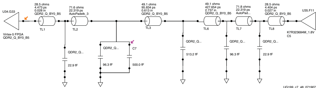
Figure 7-48: Post-Layout IBIS Schematics of QDRII Read Data Bit (QDR2_Q_BY0_B5)
