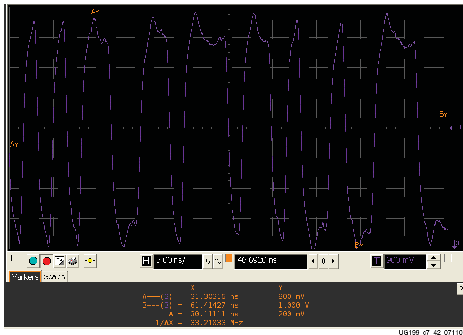
Figure 7-42: QDRII Write HW Measurement - Waveform Scope Shot at Probe Point (QDRII Memory Via)
