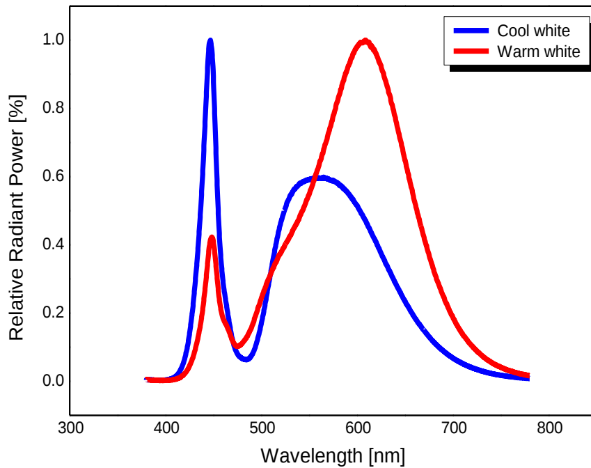
Fig 1. Color Spectrum, Ta = 25℃, IF = 350mA, RH30%
