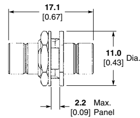
Part No. 1311127-1
