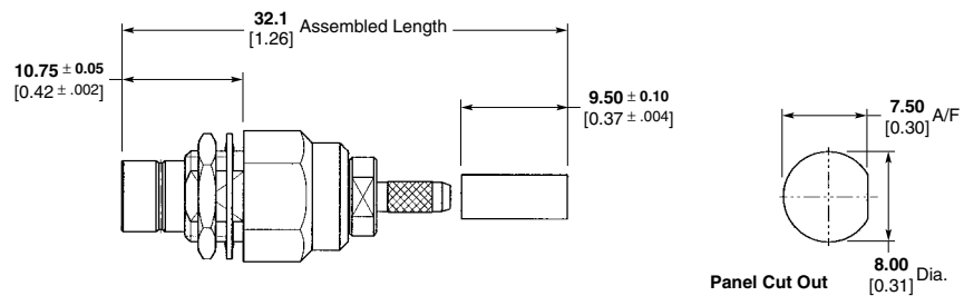
Panel Cut Out
