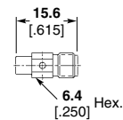
MCX Jack – SMA Jack
