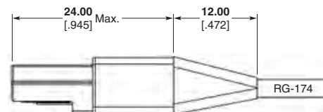
Cable Plug
