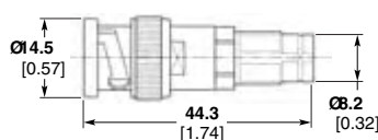
BNC Plug – Series 1.6/5.6 Jack
