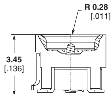
Mated Position
