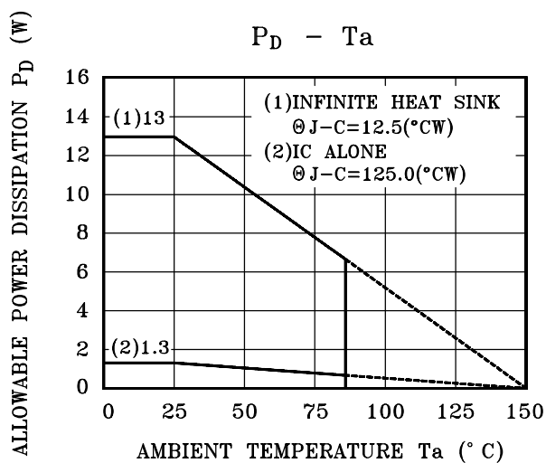
Fig 3. Power Dissipation Characteristics.
