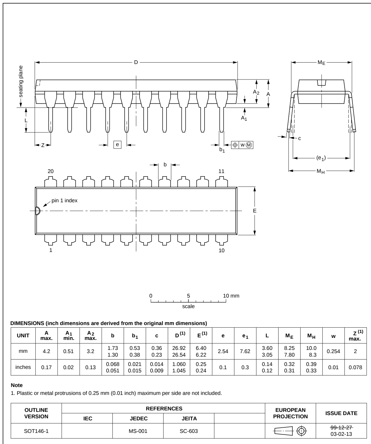
Fig 21. Package outline SOT146-1 (DIP20)
