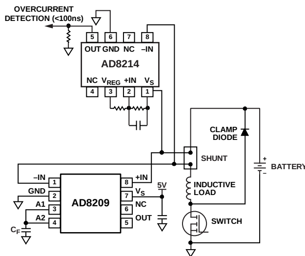
Figure 26. Battery-Referenced Shunt Resistor
