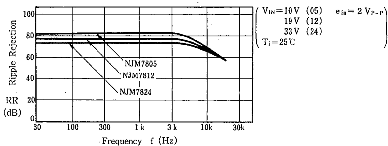
NJM7805/12/24 Ripple Rejection vs. Frequency
