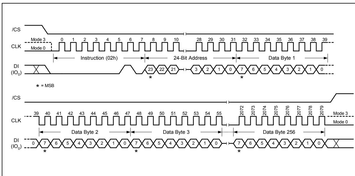
Figure 14. Page Program Instruction Sequence Diagram
