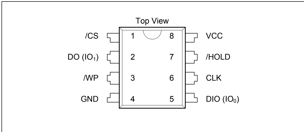
Figure 1c. W25X40BL Pin Assignments, 8-pin PDIP 300-mil (Package Code DA)
