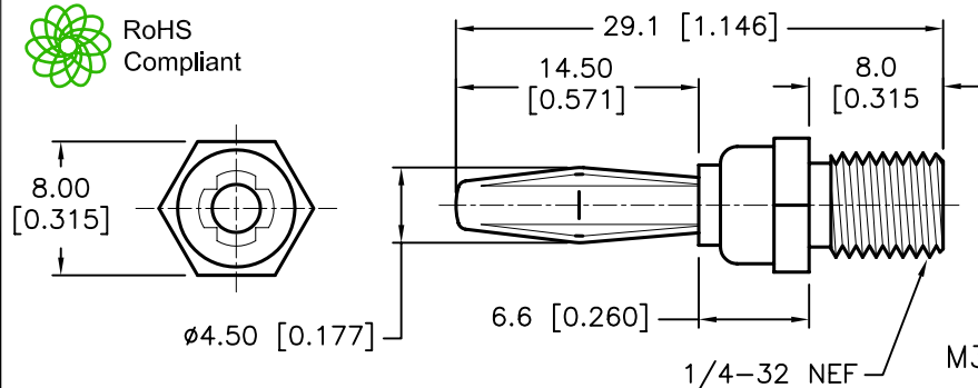
PLUG BODY
