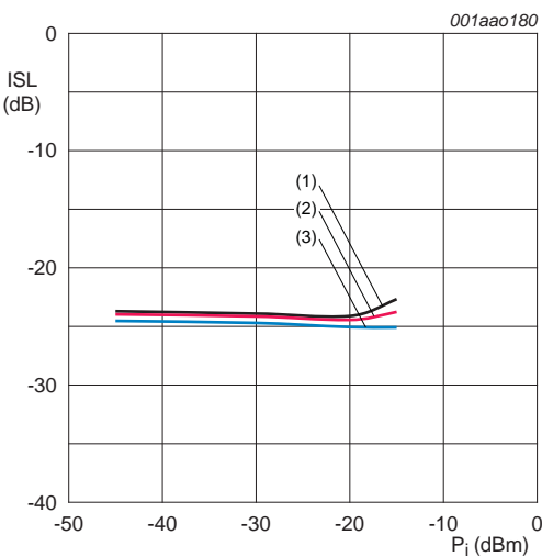
T_{\text{amb}} = 25 \text{ }^{\circ}\text{C} ; f = 1575 \text{ MHz} . (1) V_{\text{CC}} = 1.5 \text{ V} (2) V_{\text{CC}} = 1.8 \text{ V} (3) V_{\text{CC}} = 2.85 \text{ V}
