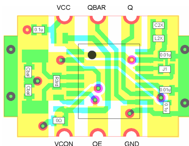
2X Layout (TSSOP)
