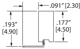
SINGLE ROW, RIGHT ANGLE (NGCN)
