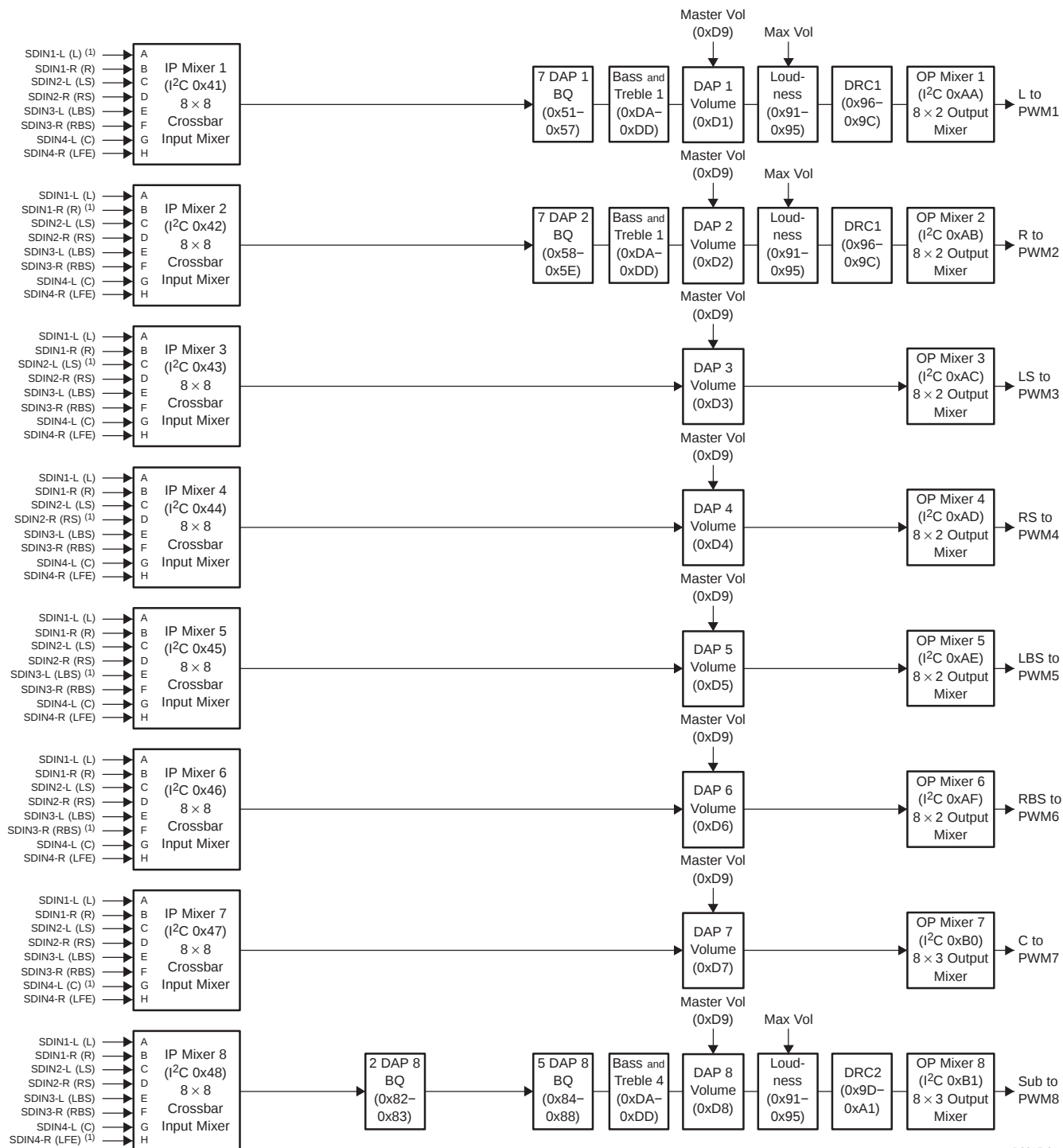
Figure 2-2. TAS5508 Architecture With I²C Registers (Fs = 176.4 kHz or Fs = 192 kHz)
