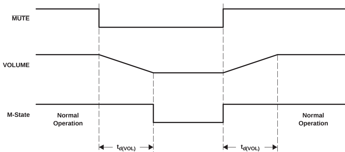
Figure 4-7. Mute Timing
