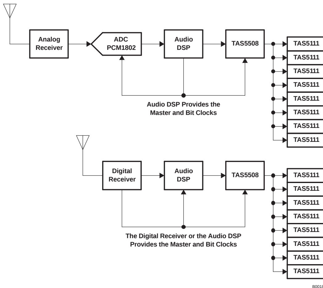
Figure 2-22. Block Diagrams of Typical Systems Requiring TAS5508 Automatic AM Interference-Avoidance Circuit
