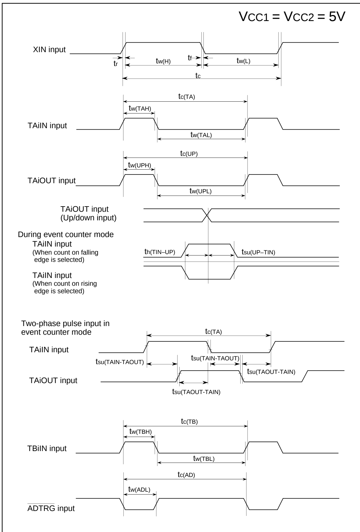
Figure 5.22 Timing Diagram (1)
