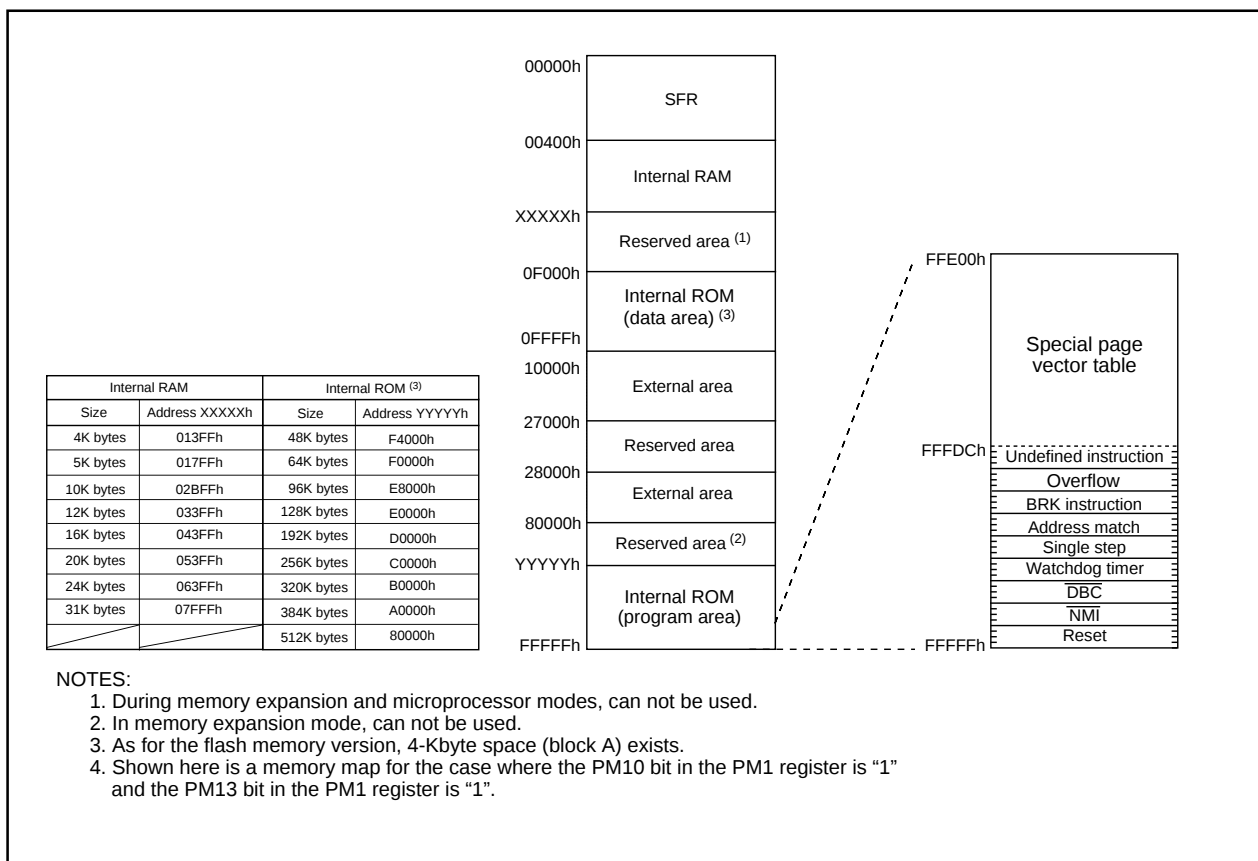
Figure 3.1 Memory Map
