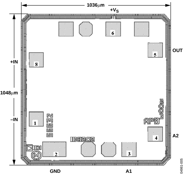
Figure 5. Metallization Photograph
