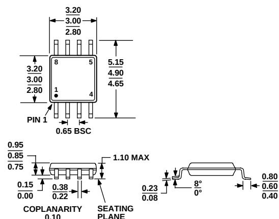
Figure 53. 8-Lead Mini Small Outline Package [MSOP] (RM-8)
