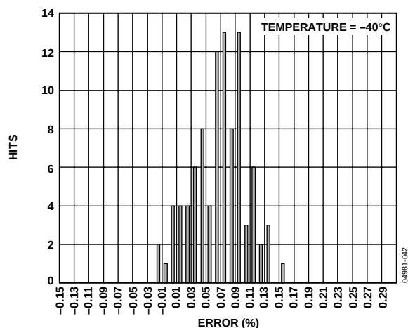
Figure 24. MSOP Gain Accuracy, Temperature = -40^{\circ}\text{C}
