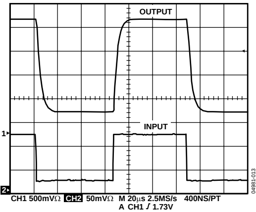
Figure 13. Pulse Response
