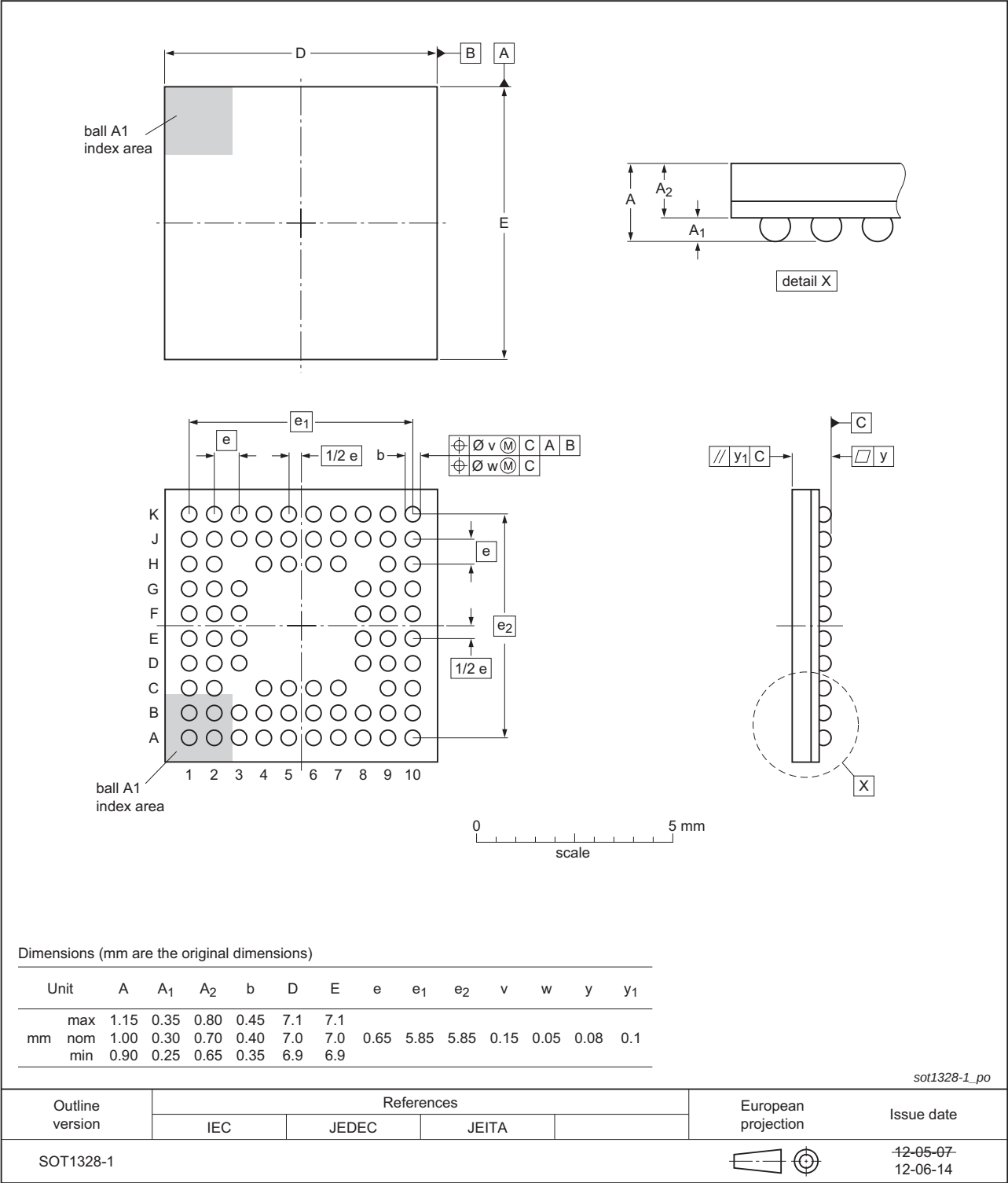
TFBGA80: plastic thin fine-pitch ball grid array package; 80 balls SOT1328-1
