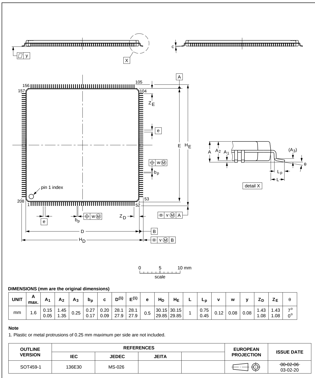
Fig 45. Package outline SOT459-1 (LQFP208)
