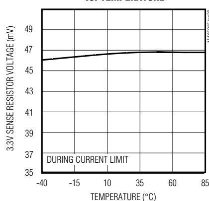
3.3V O SENSE RESISTOR VOLTAGE vs. TEMPERATURE
