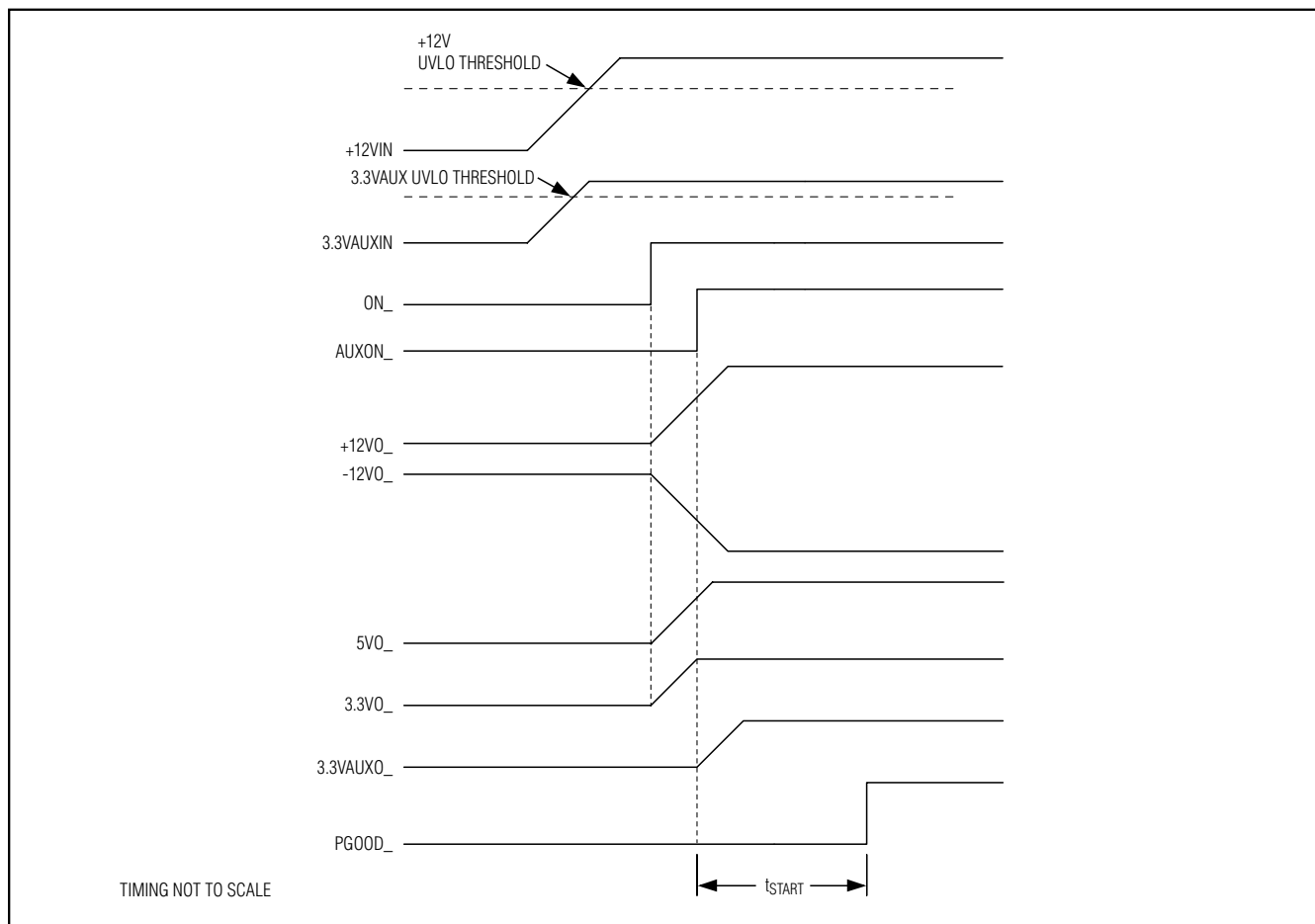
Figure 1. Startup Waveforms
