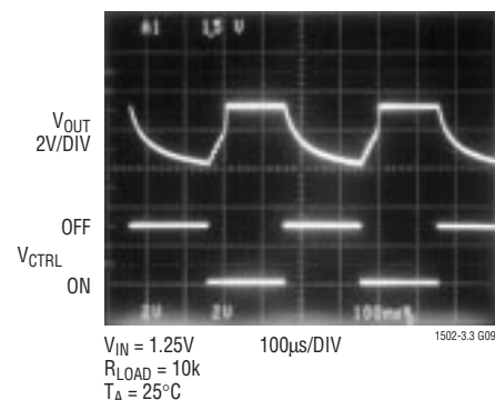
Shutdown Waveforms (See Figure 1)
